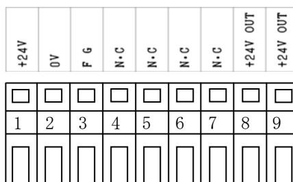
(Fig. 1 Power input terminal)
